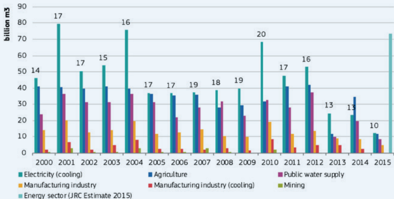
Figure 5. Historical water abstraction for energy (cooling), agriculture, public water supply, manufacturing industry, and mining reported [Eurostat 2018]. The number of MS reporting information on freshwater for energy cooling abstraction is provided for each year.
