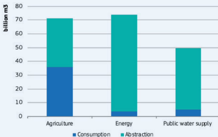
Figure 6. Comparison of water abstraction and consumption for energy (JRC analysis [Medarac et al. 2018]), agriculture (JRC analysis, [Vanham & Bidoglio 2013]), public water supply ((Eurostat 2018)).
