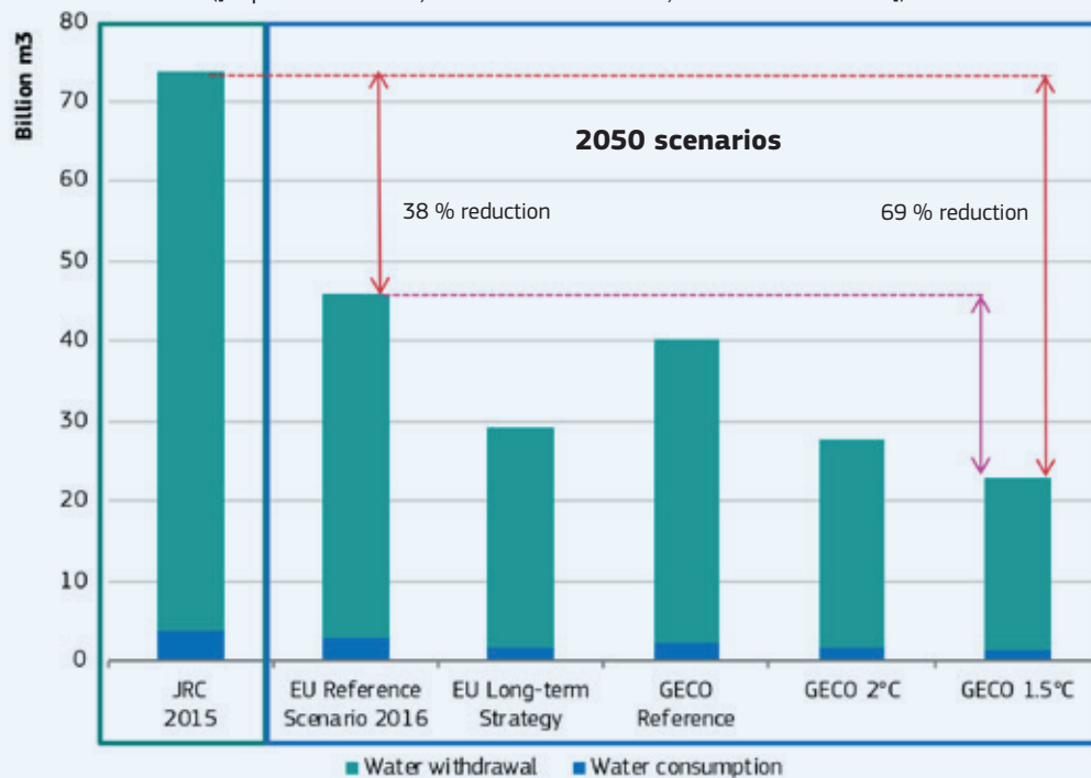
Figure 15. Alternative 2050 estimations of the projected water use by the EU energy system ([Capros et al. 2016, Keramidas et al. 2018, Medarac et al. 2018])
