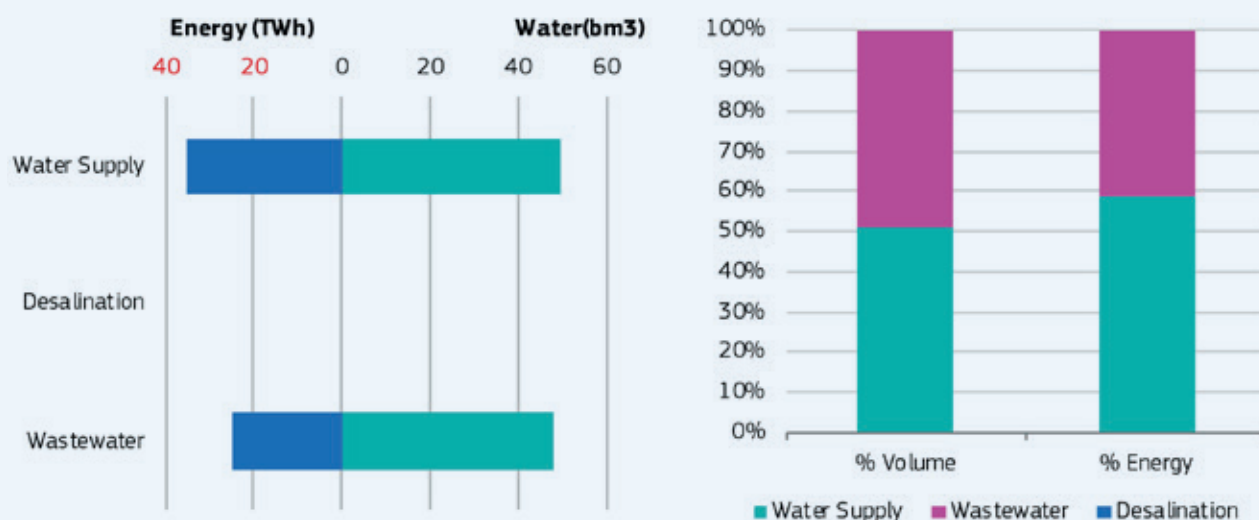
Figure 10. Energy needs for the different parts of the water sector in 2017 (source: JRC).
