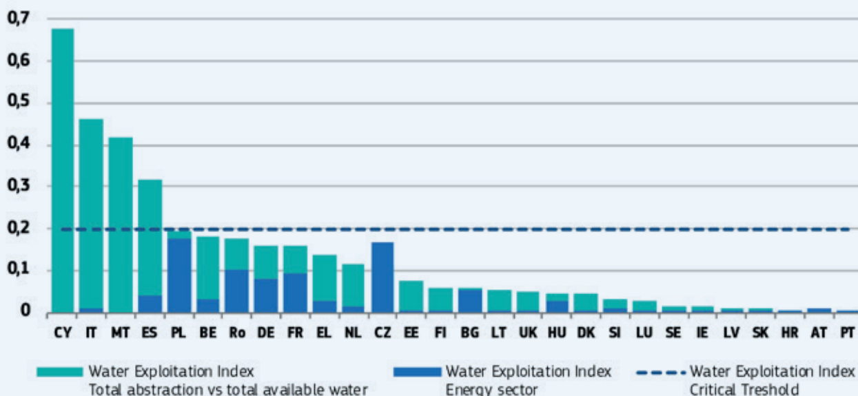
Figure 7. Water Exploitation Indexes (for energy and total) based on reported data [Eurostat 2018]
